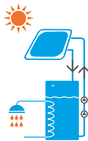
Drain-back solar system
