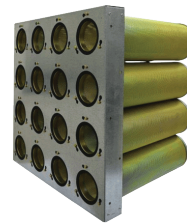
Fig 14: Carbon Canister
